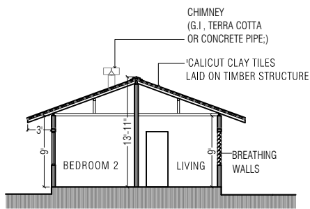
SECTION Z-Z Scale : 16ft to an inch
