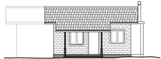
FRONT ELEVATION Scale : 1/16ft to an inch
