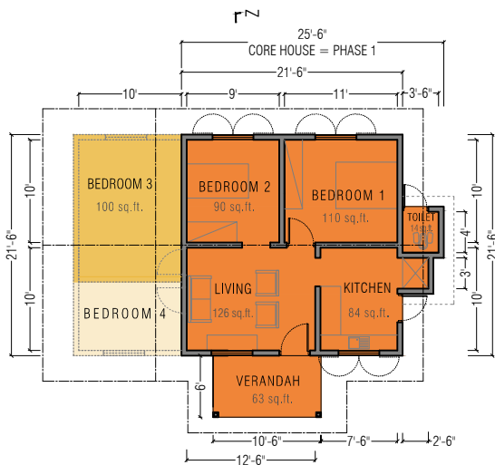
GROUND FLOOR PLAN Scale : 1/16ft to an inch
