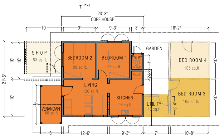
GROUND FLOOR PLAN Scale : 16ft to an inch
