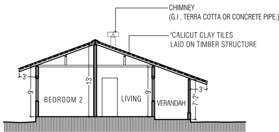
SECTION Z-Z Scale : 1/16ft to an inch
